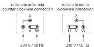
MEC 71/90 standard
